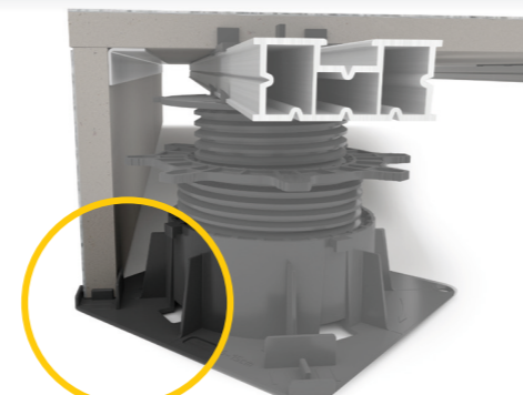
Spor/feste for fasadeplater
